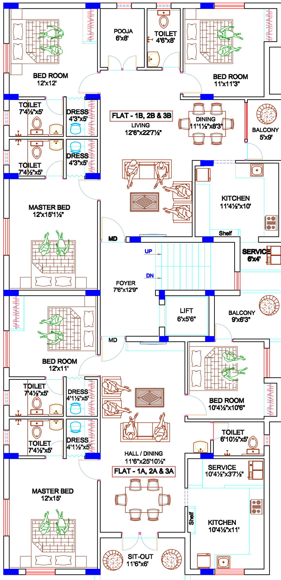
TYPICAL 1, 2 & 3 FLOOR PLAN
